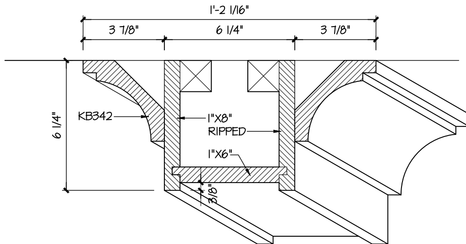
MAJOR BEAM
