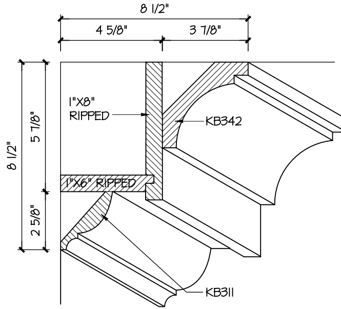
WALL BEAM
